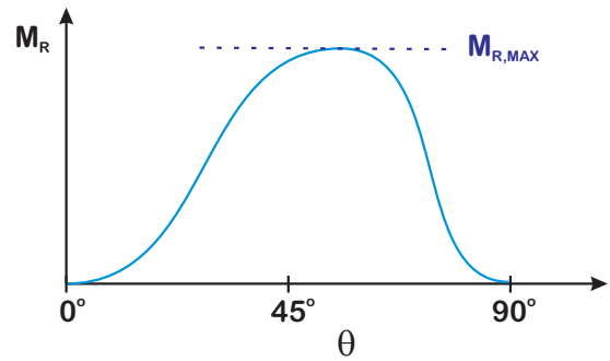
Fig. 3. A typical righting moment curve. The righting moment increases with increasing angle until some maximum value, M_{R,MAX} .
