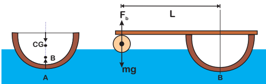
Fig. 7. An unballasted hull, made from a section of a cylinder, has generally poor roll stability. This is the case for the dugout canoe on the left. Adding an outrigger, on the right, creates a righting moment.
