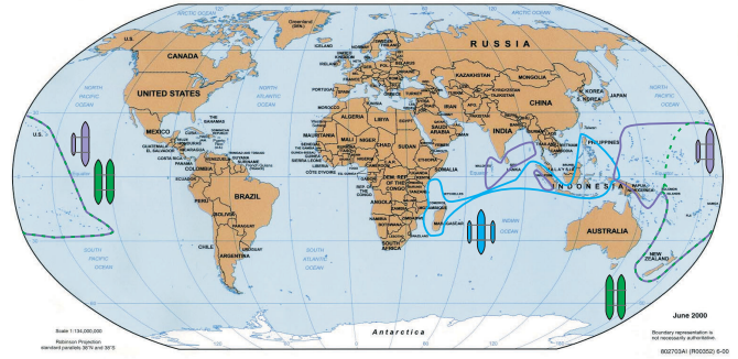
Fig. 12. The distribution of outrigger canoes across the world. Note the broader distribution of single outriggers to double outriggers. Data summarized from maps in Hornell [2] and Doran [7].
