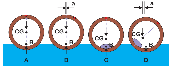
Fig. 4. A cylindrical hull has no roll stability, because the center of buoyancy is always under the center of gravity. Adding ballast at the bottom adds stability. An unballasted hull, made from a section of a cylinder, has generally poor roll stability.
