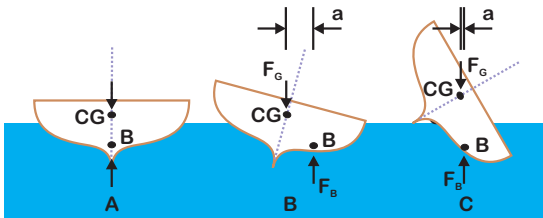
Fig. 2. Righting moment for a typical plank boat hull. (Reproduced from [6], p. 252.)
